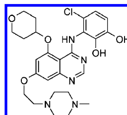
Figure 3. Catechol impurity.
